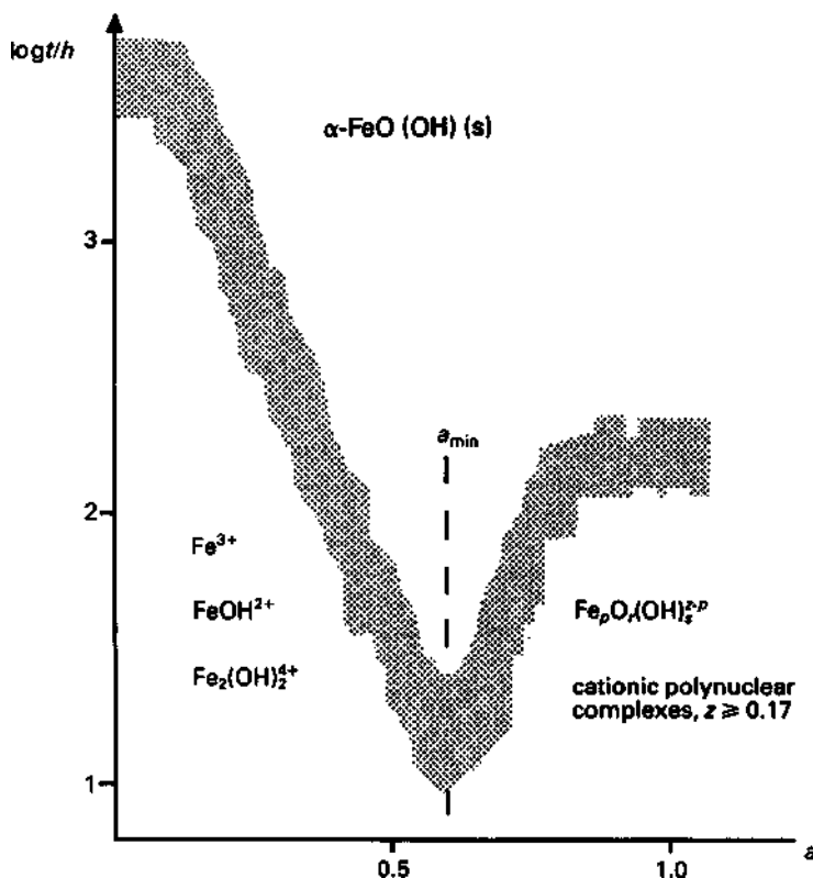
Figure 1.5 The variation of precipitation times with molar ratios of a = \text{HCO}_3^- / \text{Fe(III)} for 0.6 M iron(III) perchlorate solutions. \tau is the somewhat arbitrarily defined time elapsed before a Tyndall effect is observed. (From Crichton, 1991.)
