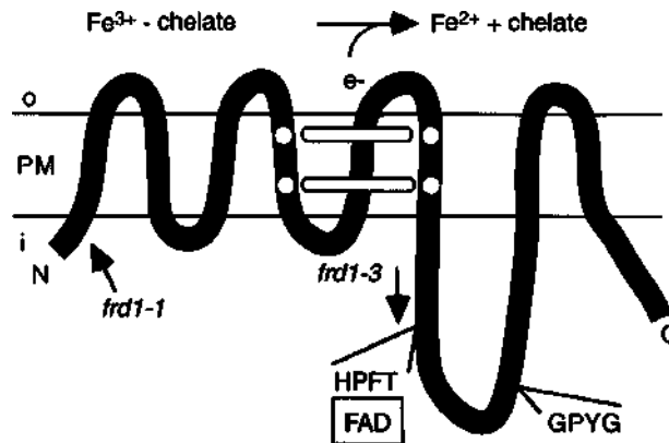
Figure 4.2 Hypothetical plasma membrane (PM)-associated structure of FRO2. Four histidine residues (white spots) predicted to coordinate two intramembrane haem groups (white bars) are indicated, as are the tetrapeptide binding sites for FAD and NAD(P)H. The sites of mutations in the FRO gene are indicated ( frd1-1 , frd1-3 ); i, inside cell; o, outside cell. Reprinted with permission from Nature (Robinson et al. , 1999). Copyright (1999) Macmillan Magazines Limited.
